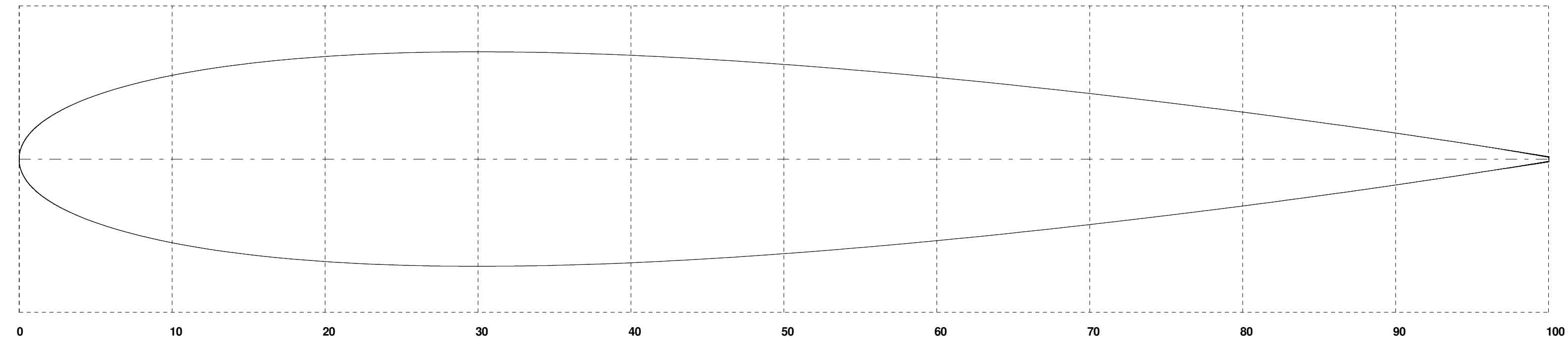
RIB 1 Chord (millimetres) : 410.000 L.E. Ref. Distance (millimetres) : 0.000 C.L. Ref. Distance (millimetres) : 209.750
