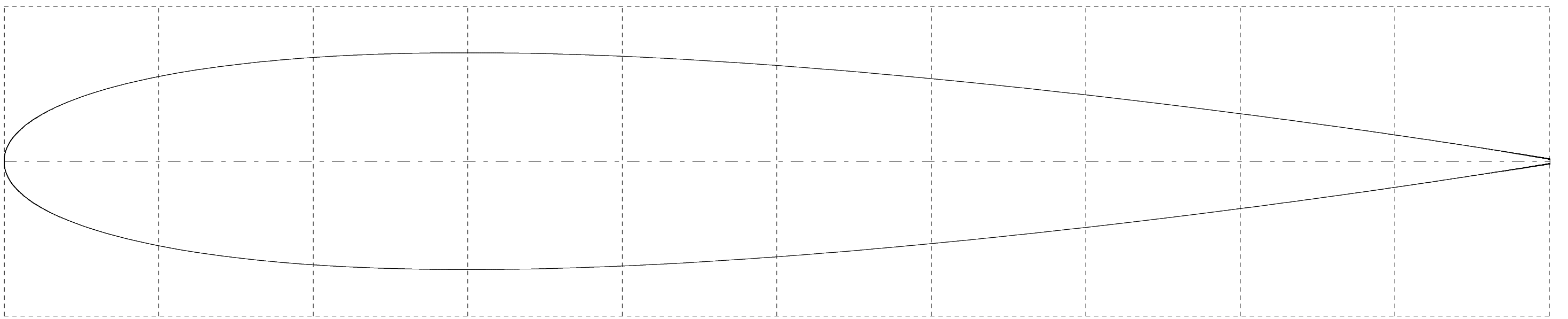
RIB 3 Chord (millimetres) : 383.333 L.E. Ref. Distance (millimetres) : 26.667 C.L. Ref. Distance (millimetres) : 629.250
