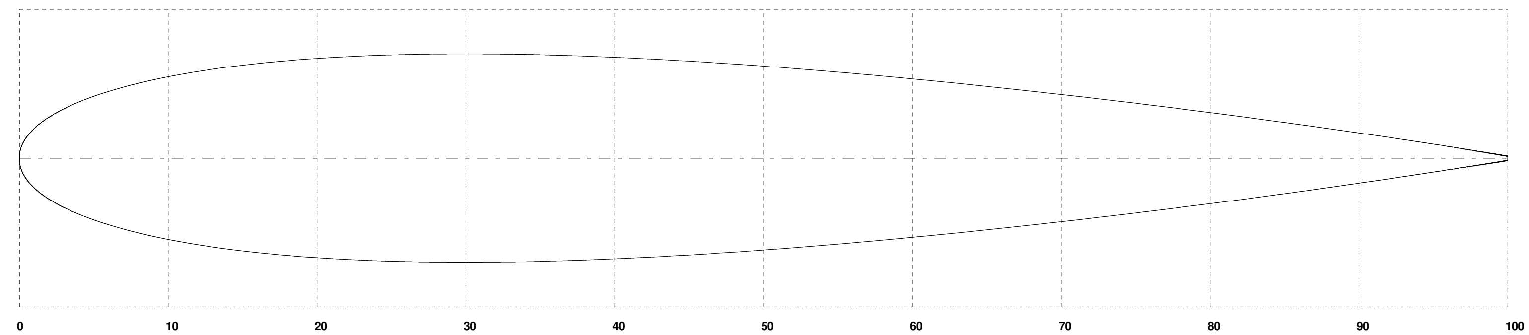
RIB 2 Chord (millimetres) : 396.667 L.E. Ref. Distance (millimetres) : 13.333 C.L. Ref. Distance (millimetres) : 419.500
