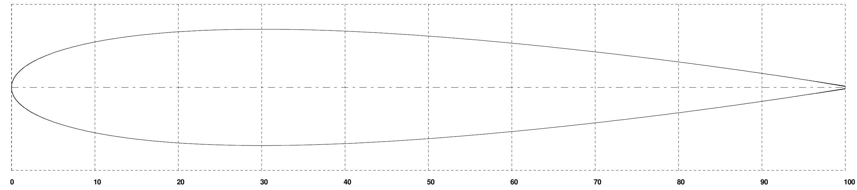
RIB 4 Chord (millimetres) : 370.000 L.E. Ref. Distance (millimetres) : 40.000 C.L. Ref. Distance (millimetres) : 839.000
