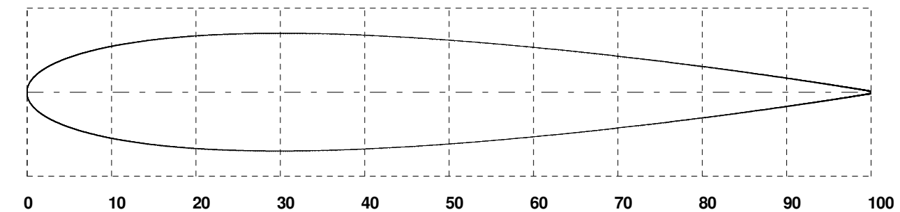
RIB 3 Chord (millimetres) : 160.000 L.E. Ref. Distance (millimetres) : 210.000 C.L. Ref. Distance (millimetres) : 460.000
