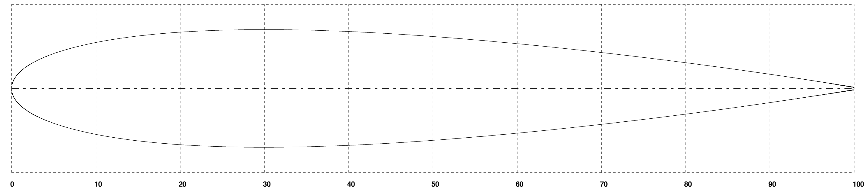
RIB 1 Chord (millimetres) : 370.000 L.E. Ref. Distance (millimetres) : 0.000 C.L. Ref. Distance (millimetres) : 153.333
