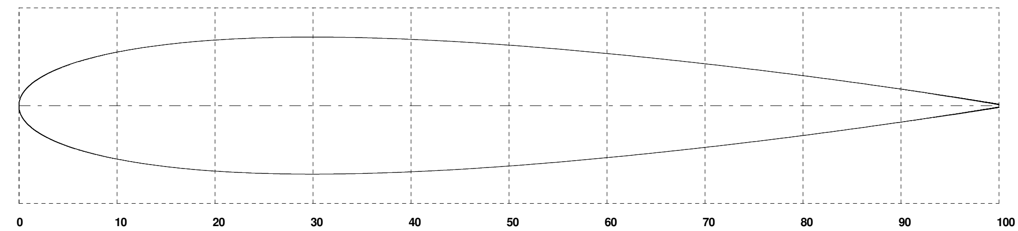
RIB 2 Chord (millimetres) : 265.000 L.E. Ref. Distance (millimetres) : 105.000 C.L. Ref. Distance (millimetres) : 306.667
