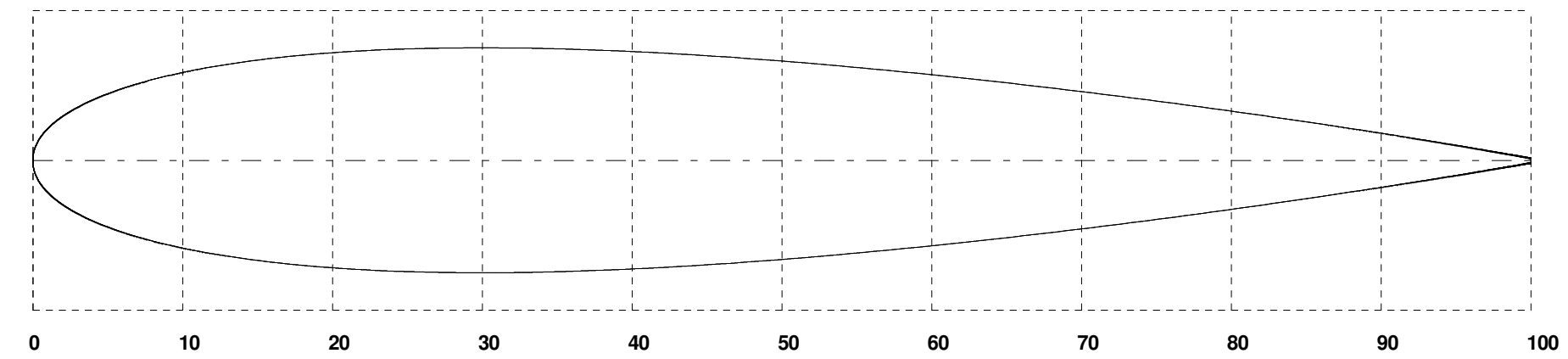
RIB 3 Chord (millimetres) : 233.667 L.E. Ref. Distance (millimetres) : 37.333 C.L. Ref. Distance (millimetres) : 678.750
