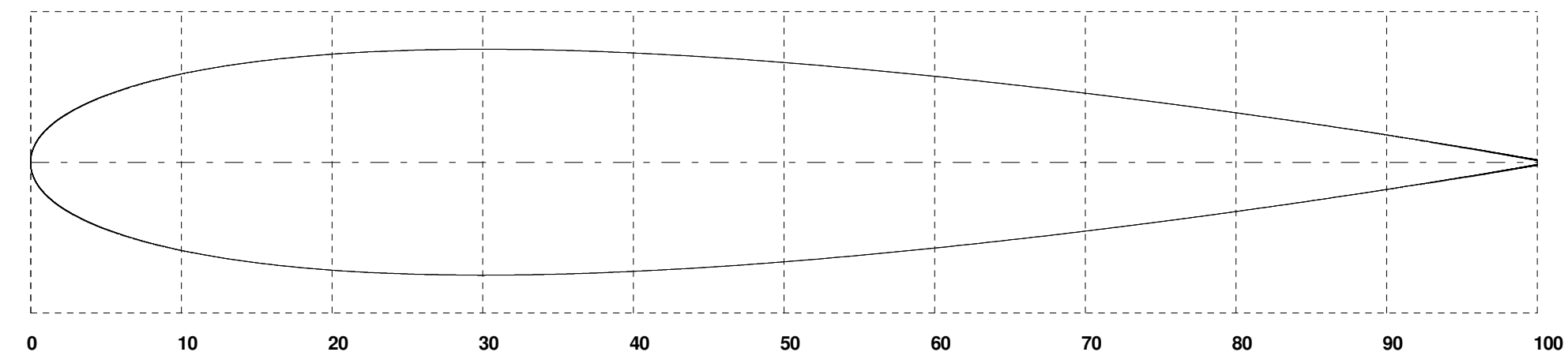
RIB 2 Chord (millimetres) : 252.333 L.E. Ref. Distance (millimetres) : 18.667 C.L. Ref. Distance (millimetres) : 452.500
