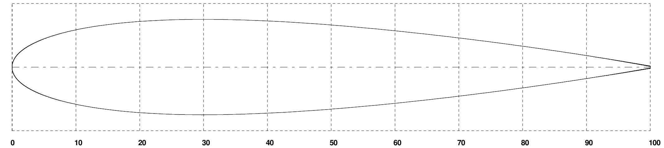
RIB 1 Chord (millimetres) : 271.000 L.E. Ref. Distance (millimetres) : 0.000 C.L. Ref. Distance (millimetres) : 226.250
