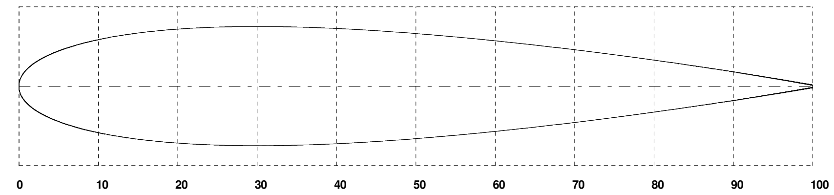
RIB 4 Chord (millimetres) : 215.000 L.E. Ref. Distance (millimetres) : 56.000 C.L. Ref. Distance (millimetres) : 905.000
